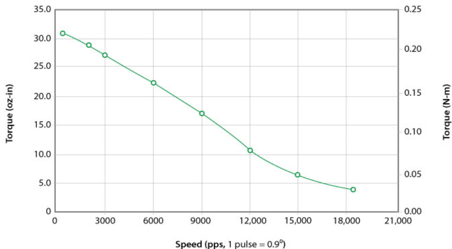
4418X-01 24VDC, 1.5 Amps/Phase, Bipolar, 1/2 Stepping
